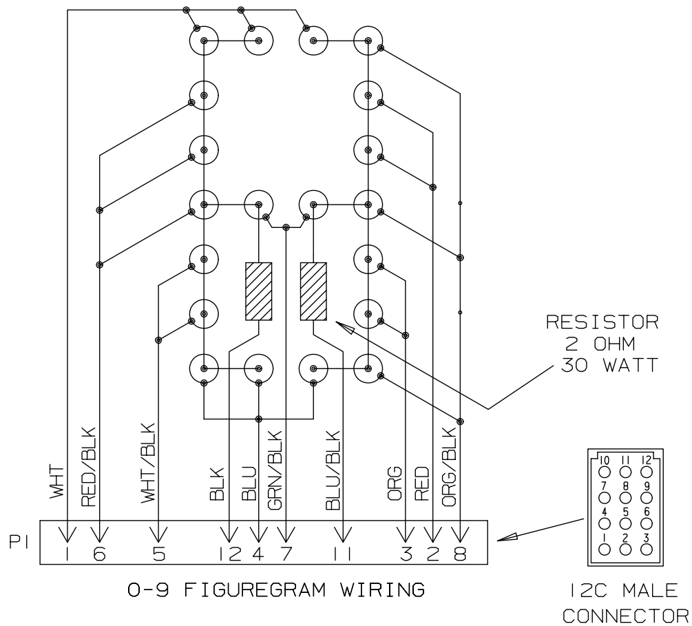
8 BIT FIGUREGRAM WIRING
