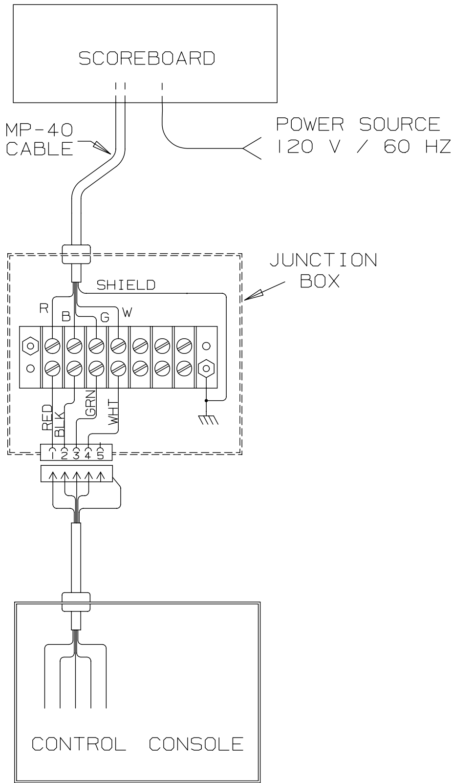
SYSTEM LAYOUT
