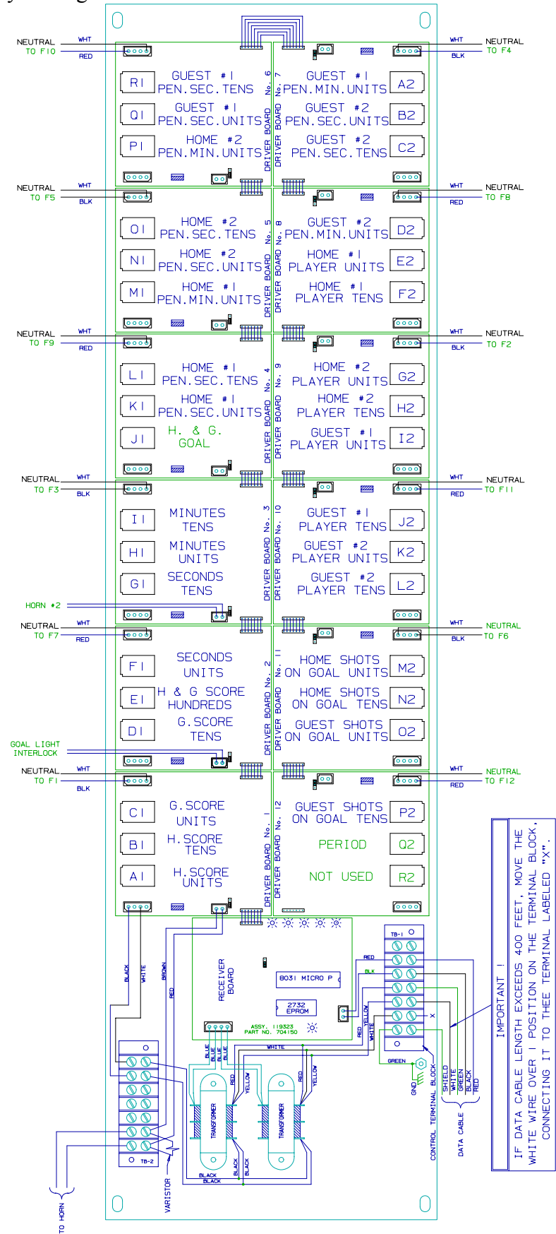
CONTROLLER ASSEMBLY
